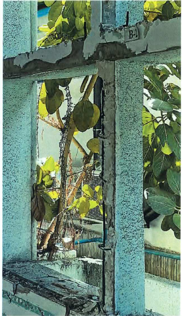
Figure 10 RC Column, spalling damage
