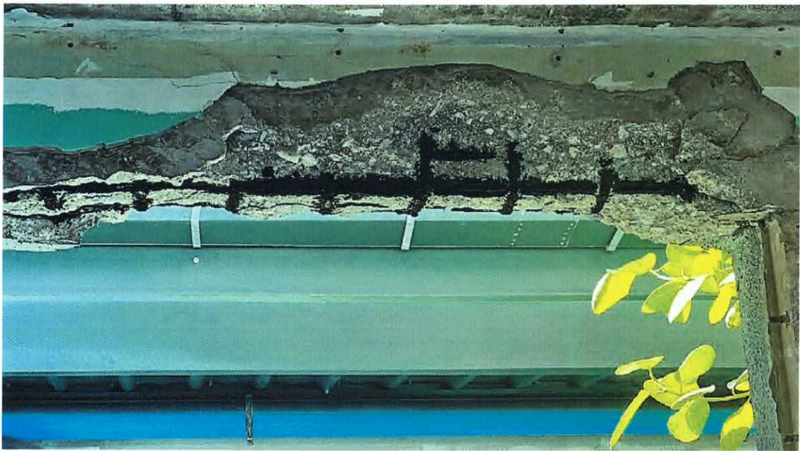
Figure 13 RC Beam, spalling damage.
